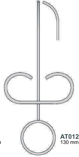
YUKARI EĞRİ CURVED UP Ø 1,8 mm
